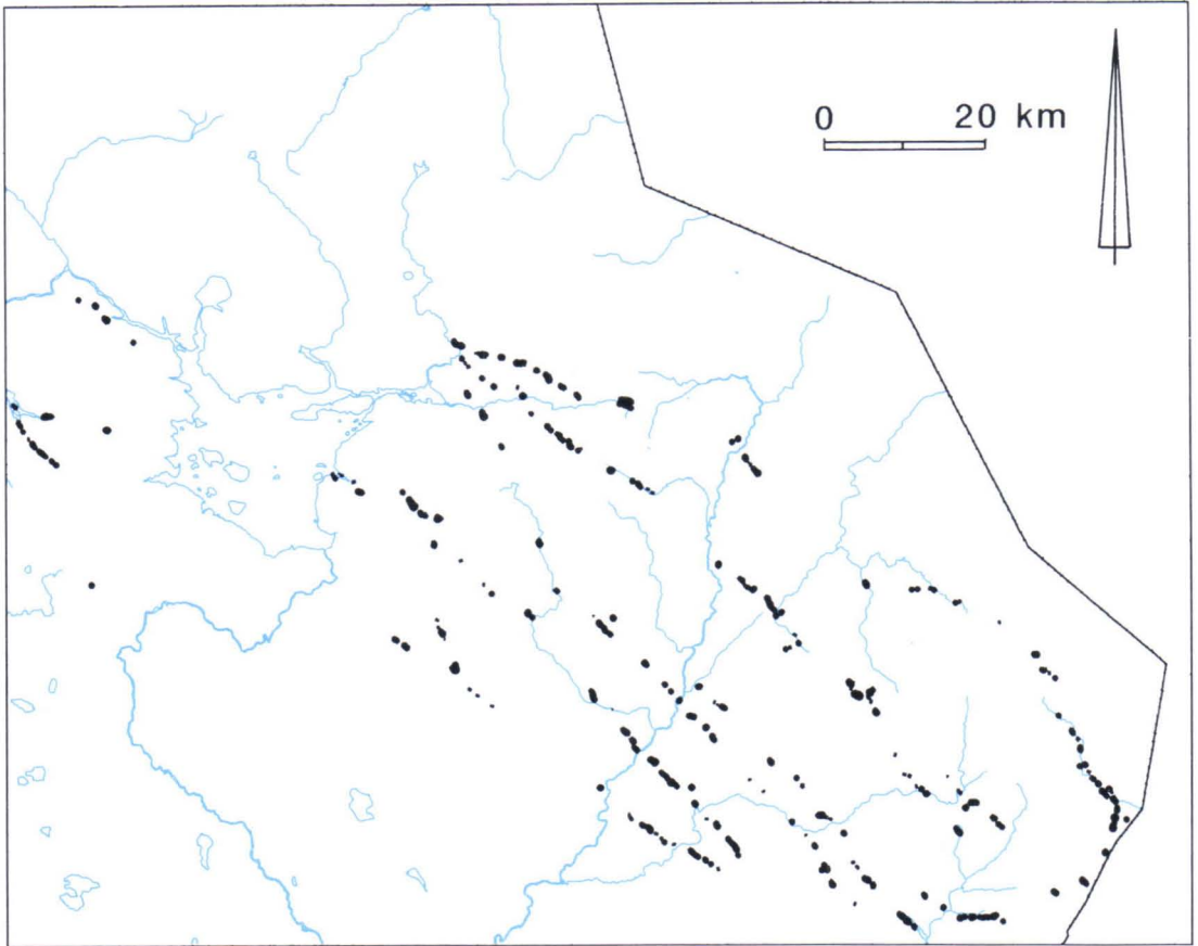
Fig. 21. Subglacial esker chains oriented in a NW-SE direction.
