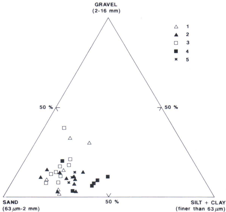
Fig. 4. Ternary diagram of the grain-size distribution of till units in the Martti-Ruuvaaja area. 1 = surficial till, 2 = youngest till unit, 3 = younger till unit, 4 = 'Old Northern' till unit, 5 = oldest till unit.
