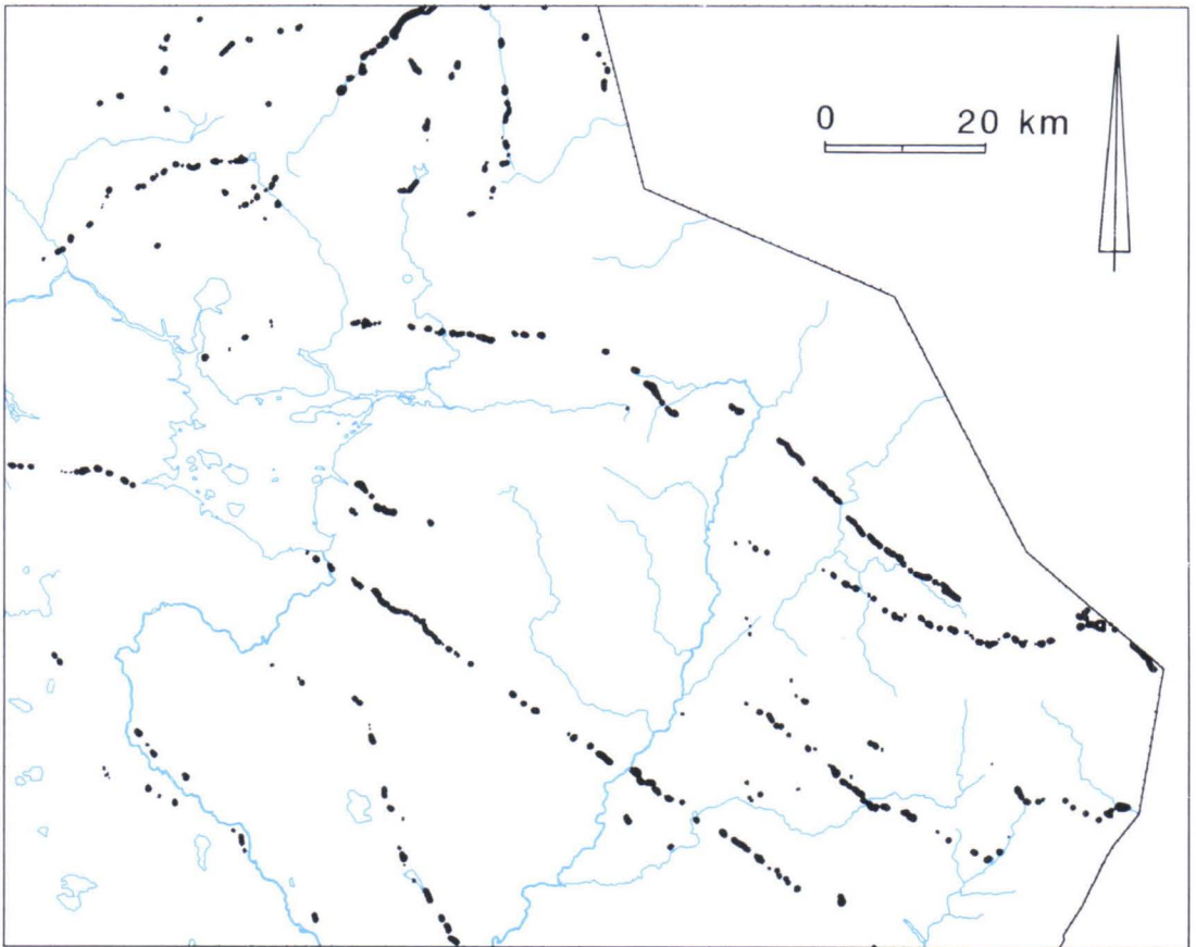
Fig. 17. Subglacial esker chains without till cover.
