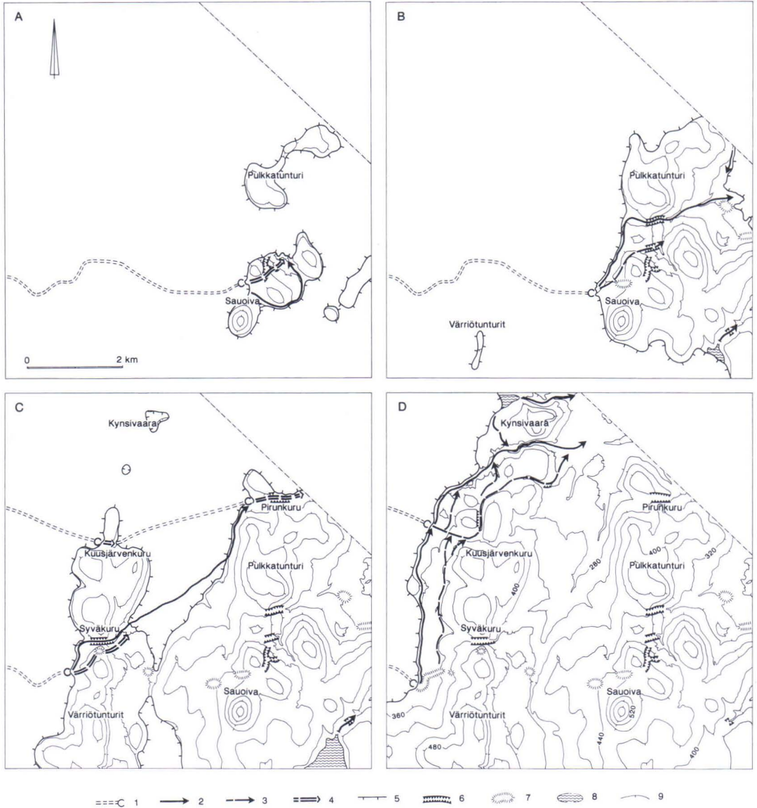
Fig. 9. Glaciohydrographic history of the Värriötunturit-Sauoiva area and disappearance of the glacier (A-D): 1 = subglacial meltwater system and its mouth, 2 = functioning proglacial or marginal channel, 3 = former proglacial or marginal channel, 4 = former subglacial channel, 5 = ice margin, 6 = gorge, 7 = esker, 8 = ice-dammed lake, 9 = contour line.
