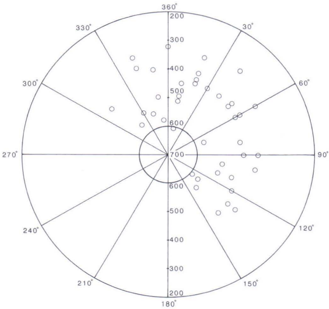
Fig. 32. Flutings on the slope of Siliäselkä, north of Lake LUIROJÄRVI.
