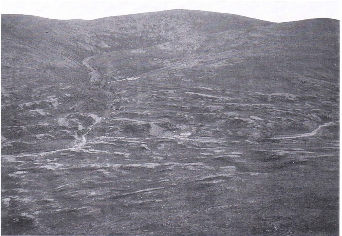
Fig. 40. Hummocky moraines in the Sarvijoki river valley. Laterally formed ridges are seen on the slopes and unoriented hummocks on the valley floor.
