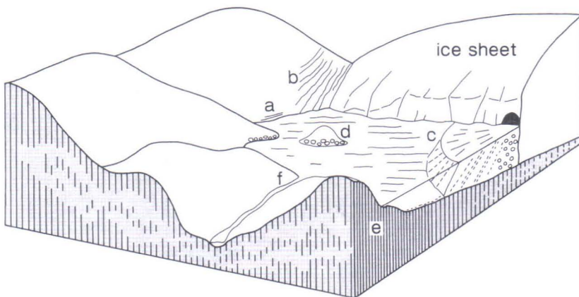
Fig. 24. Types of ancient shorelines and other marks of former ice lakes. a = washed bedrock surface, b = lateral drainage channels terminating at the surface level of the ice lake, c = delta deposited at the surface level of the ice lake, d = stone belt, e = scarp shore, f = spillway with threshold point.
