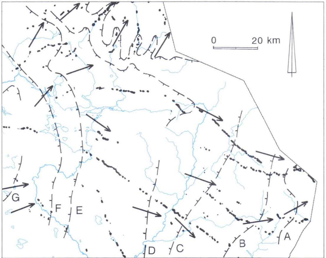
Fig. 42. Map of the retreat of the ice margin (stages A-G) and subglacial esker chains without till cover. The arrows indicate directions of ice flow during deposition of the younger till unit.
