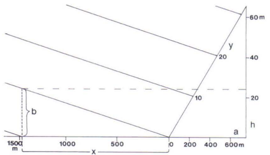
Fig. 16. A diagram showing the distance between lateral drainage channels projected on the horizontal plane allows the annual rate of thinning of the ice sheet and the distance of its retreat to be calculated. a = horizontal length of slope, h = vertical height of slope, y = number of lateral drainage channels on slope, b = thinning of glacier in metres per ten years, x = distance of ice retreat per ten years.
