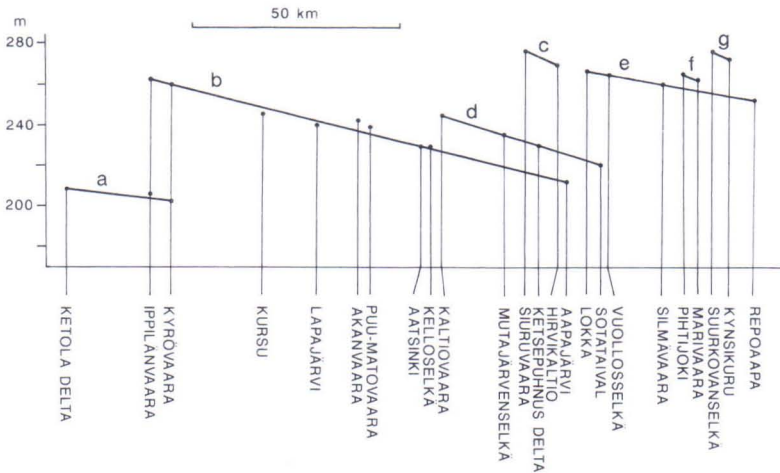
Fig. 26. Distance diagram depicting raised shore levels of the ice-dammed lakes and the Ancylus Lake in Finnish Lapland. For locations of the ice lakes, see Appendix. a = Ancylus Lake, b = Salla Ice Lake, c = Värriöjoki Ice Lake, d = combined ice lakes of Värriöjoki and Kemihaara, e = Pososaapa Ice Lake, f = Pihtijoki Ice Lake, g = Sokli Ice Lake.
