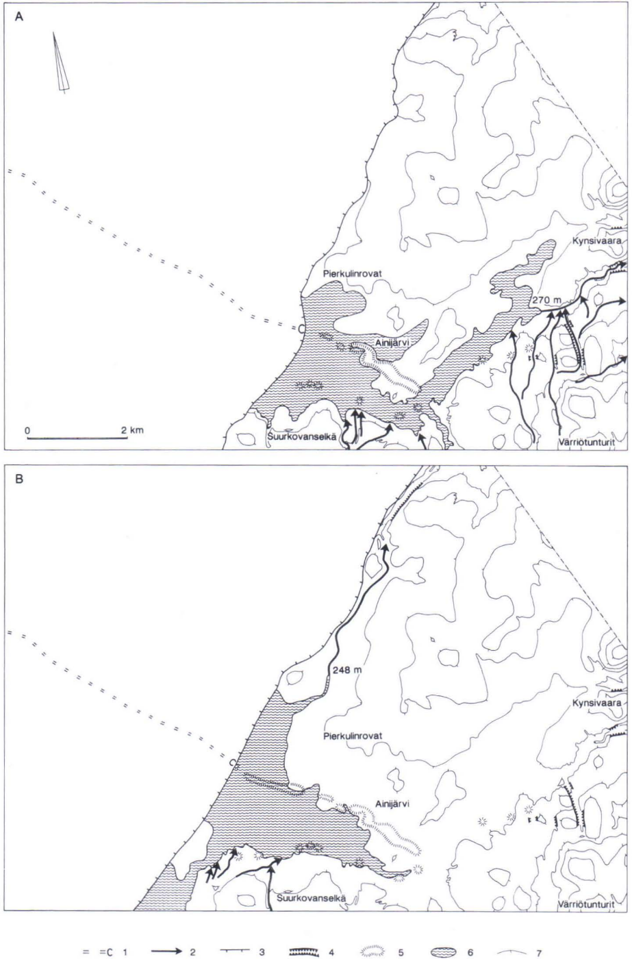
Fig. 34. History of the Sokli Ice Lake. 1 = subglacial meltwater system and its mouth, 2 = functioning proglacial or marginal channel, 3 = ice margin, 4 = gorge, 5 = esker, 6 = ice-dammed lake, 7 = contour line. The figure shows the meltwater channels emptying into the ice lake and terminating at its shore level. The altitude data refer to the threshold that regulated the water level in the ice lake.
